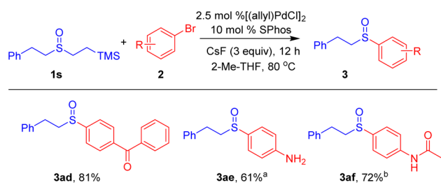
Scheme 10. Palladium Catalysed Alkyl Aryl Sulfoxide Formation with 1s
