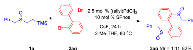
Scheme 12. Bis-Sulfoxide 3ag Formation via Palladium Catalyzed Cross-Coupling of 1a and 2ag
