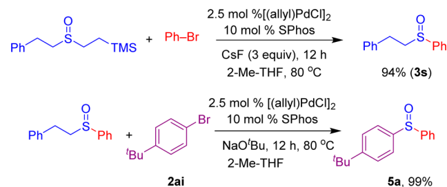
Scheme 14. Palladium Catalyzed Diaryl Sulfoxide (5a) Formation in the Presence of NaO t Bu
