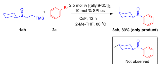
Scheme 13. Palladium Catalyzed Reaction of cis -2-(Trimethylsilyl)ethyl (4-Methyl)cyclohexyl Sulfoxides (1ah) and Bromobenzene (2a)
